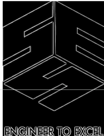
Laplacian (8-Neighbor)
